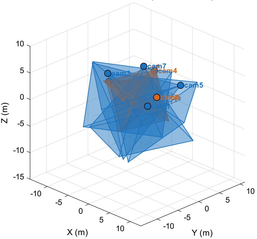
GA-best — 7 cams (Cost: 0.0185)
